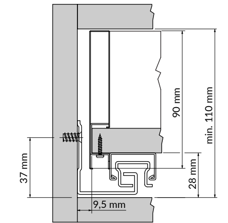
Implantation avant Front drilling and installation
