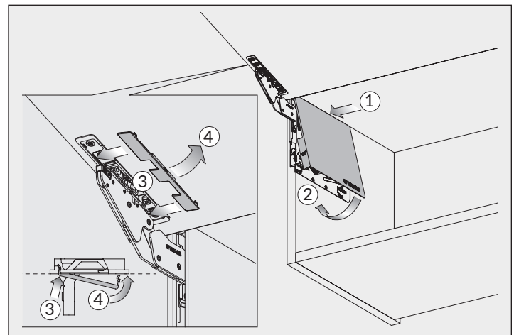
Montage des caches Cover caps application
