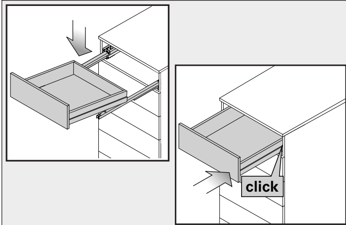
Tirer les coulisses, mettre le tiroir dessus et refermer. Extend the slides, put the drawer on them and close it.
