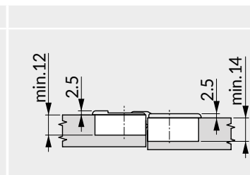
Dimensions boîtier Overall dimensions
