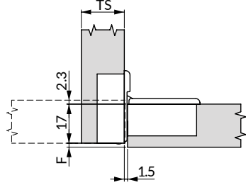
Recouvrement de 17 mm Overlay of 17 mm
