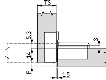
Recouvrement, 2 espaceur de 1.5 mm (2x) Overlay with two 1.5 mm spacer
